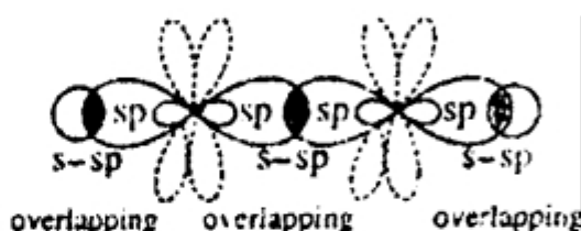
An sp-hybridized atom
