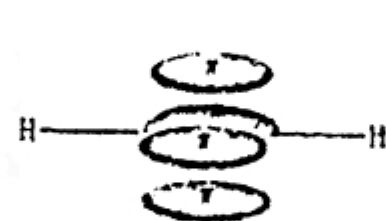
formation of π bonds
