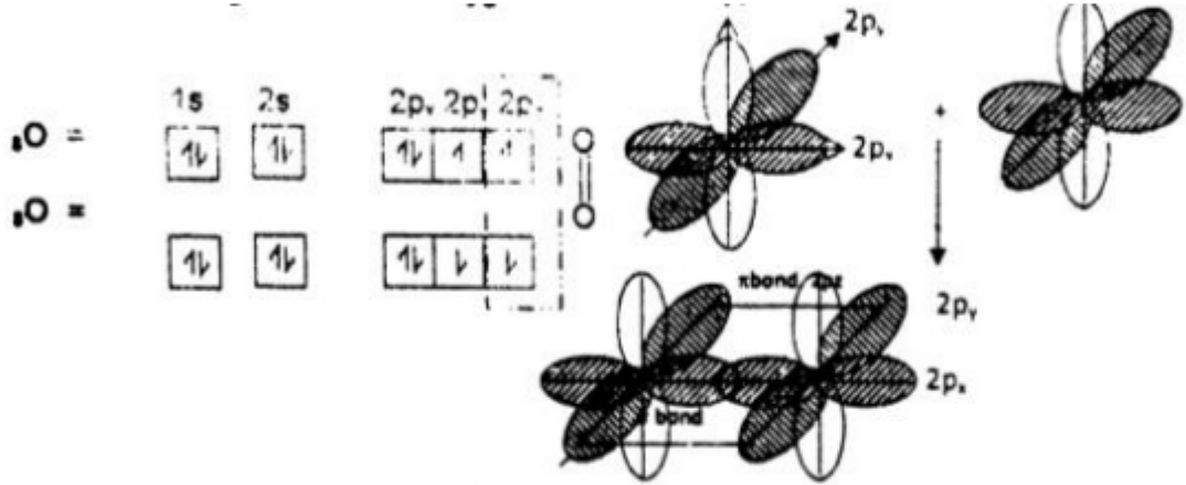
Orbital diagram of \text{O}_2
