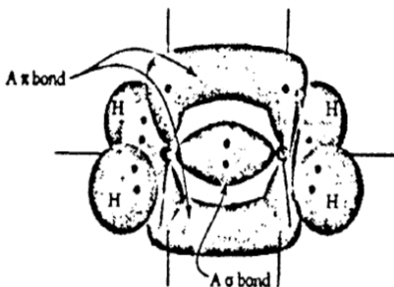
Structure of Ethene ( CH_2=CH_2 )
